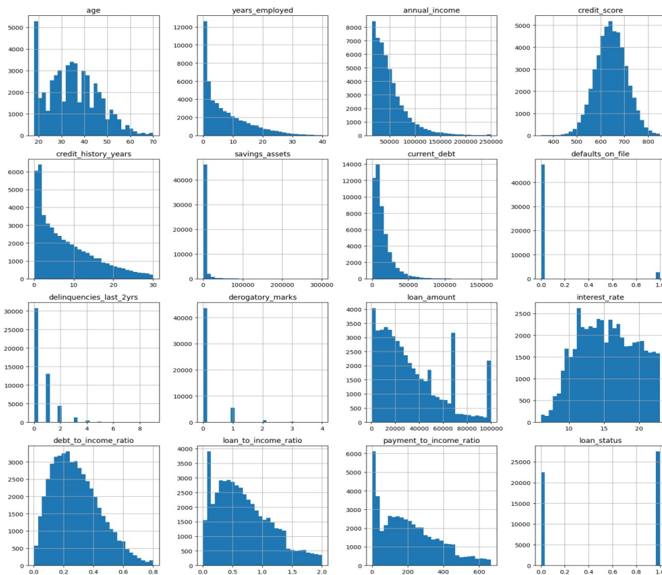
Figure 4.2 – Distributions and histograms of all features
