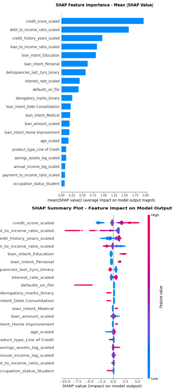
Figures 5.1 — Global Feature Importance Based on Mean Absolute SHAP Values
