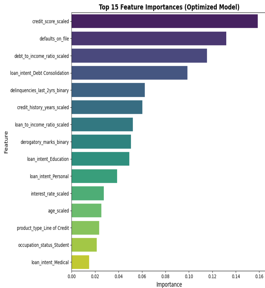
Figure 5.5 — Top 15 XGBoost feature importances for the final model
