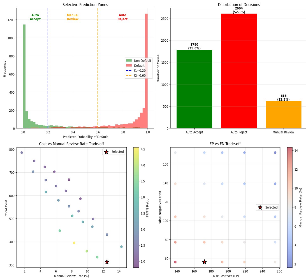
Figure 5.7 — Predicted-probability distribution with selective-prediction decision zones
