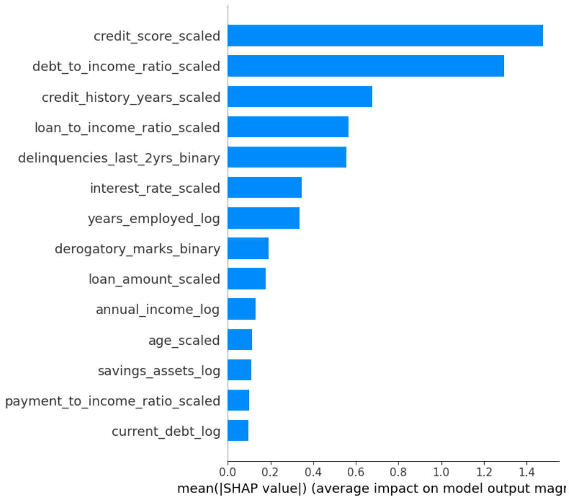
Figure 3.6 — Global SHAP Feature Importance Based on Mean Absolute Shapley Values
