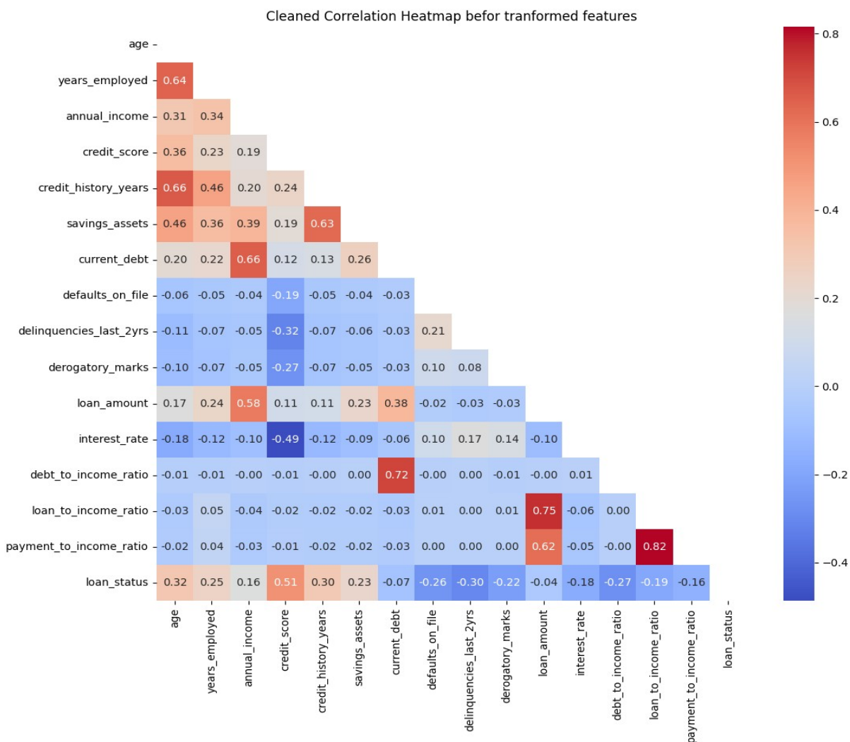
Figure 4.1 — Spearman correlation heatmap of numerical features
