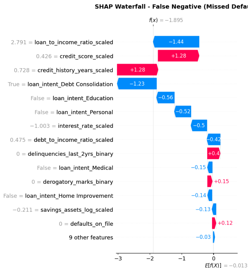
Figure 4.5 — SHAP waterfall plot for a representative false-negative applicant
